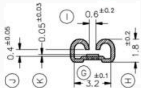
Secc. Y-Y'
