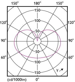
Light Distribution Diagram - LED classic 150W A67 E27 CDL FR ND 1SRT4
