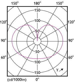
Light Distribution Diagram - LED classic 120W G120 E27 CDL FRND 1PF/4
