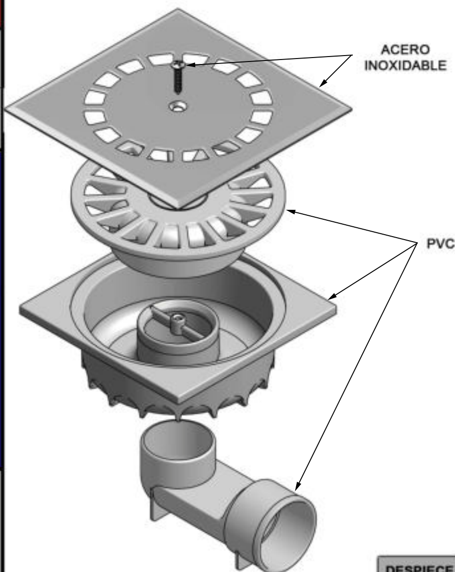
DESPIECE
