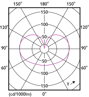
Light Distribution Diagram - LED classic 120W A67 E27 CDL FR ND 1SRT4
